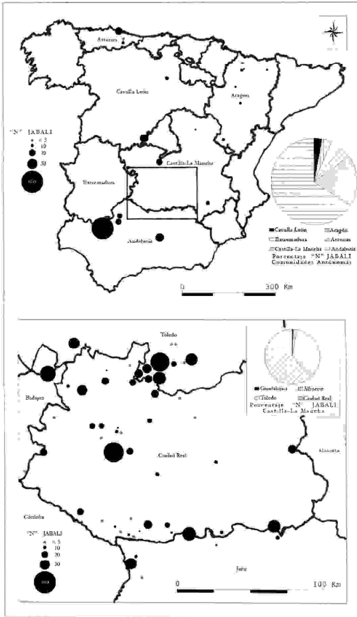
Figure 1. The location of sampling sites used in the study of wild boar in Spain. Circle diameters indicate sample size. Grey circles indicate sampling sites that had \geq 5 samples. The two diagrams show the distribution of samples among autonomous communities in Spain and between provinces in the Community of Castilla – La Mancha, respectively.
